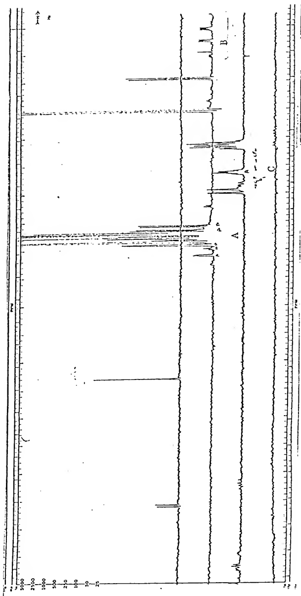
Figure 68 - ^{19}\text{F} NMR of \text{CH}_3\text{CH}_2\text{OCF}_2\text{CF}=\text{CHCH}_2\text{CF}_3
